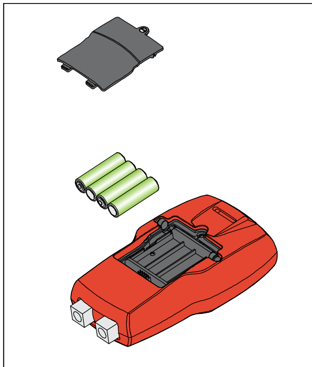
Figure 8. Battery Replacement
