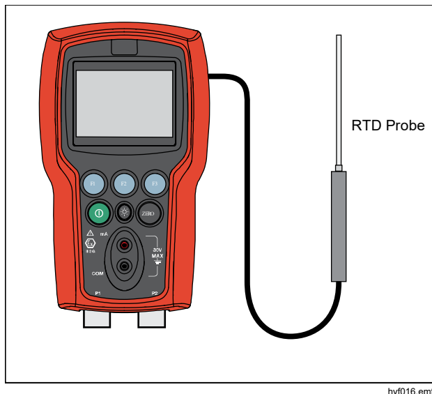
Figure 5. Temperature Measurement with RTD Probe
