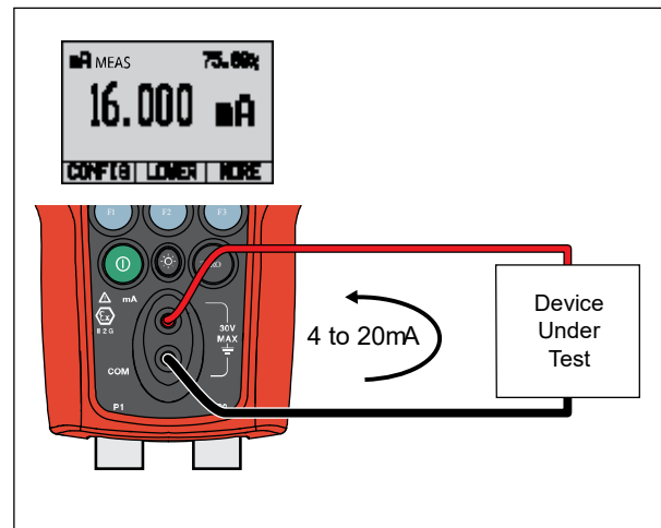
Figure 6. Measure Current
