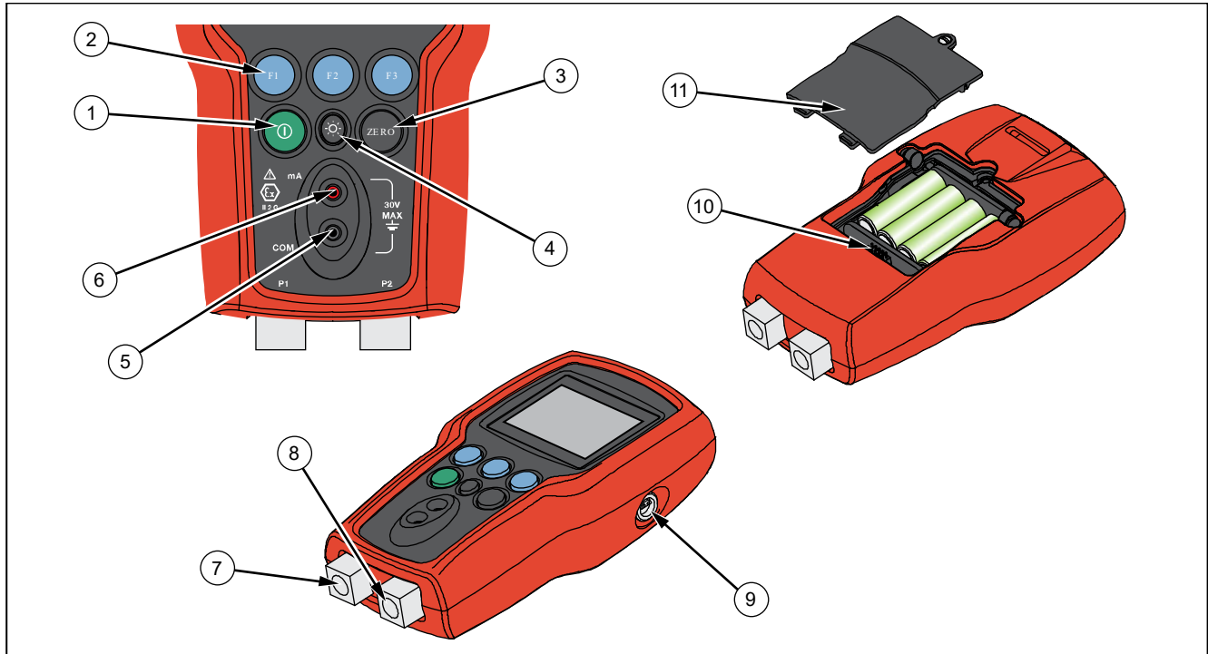
Figure 1. Product Interface
