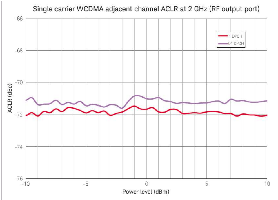
Figure 4. Single carrier W-CDMA adjacent channel ACLR versus power level at 2 GHz, RF output port
