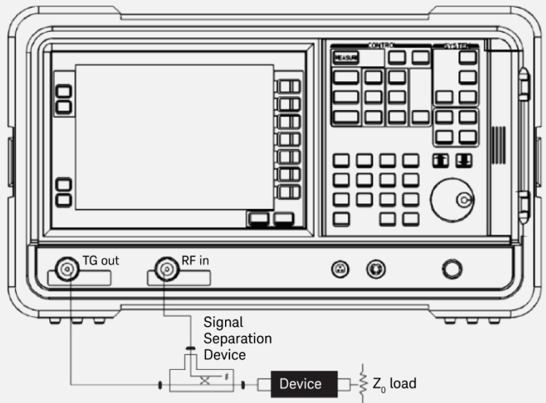
Figure 2. Conventional test setup requires an external bridge
