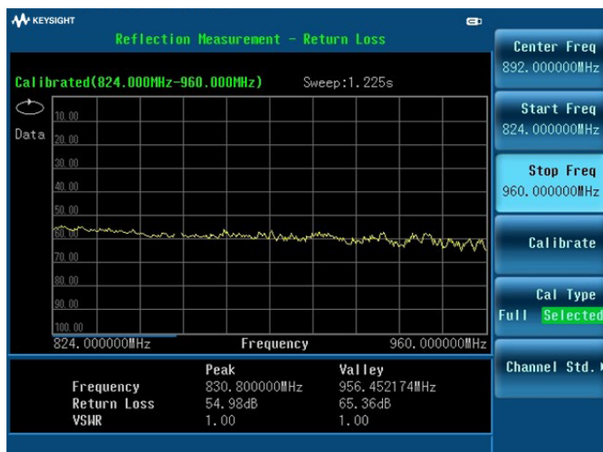
Figure 7. The calibrated N9321/22C BSA ready for measuring return loss/VSWR
