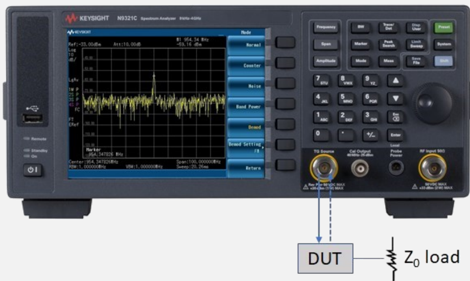
Figure 3. Simple test setup with N9321/22C BSA
