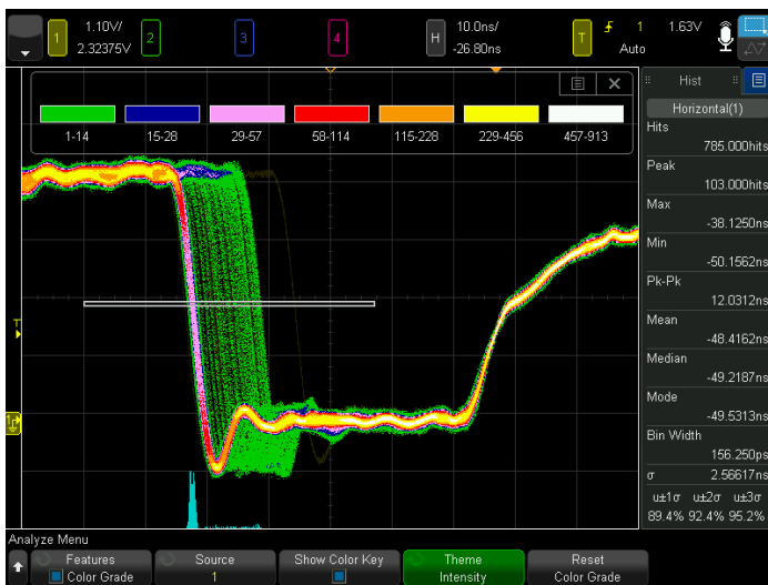
Figure 15. Color grade and histogram on a jittery clock edge.
