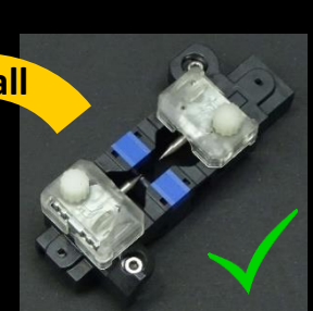
Spare V-groove with stabilized electrodes
